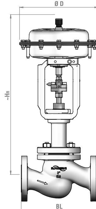
Valve with Extension Bonnet and Pneumatic Actuator
