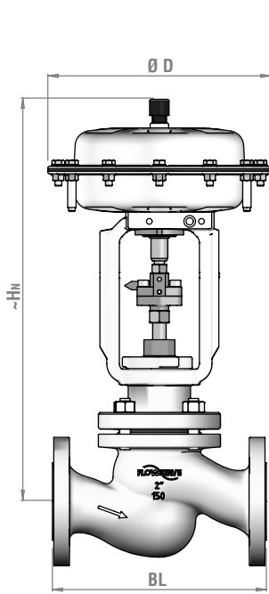
Valve with Standard Bonnet and Pneumatic Actuator
