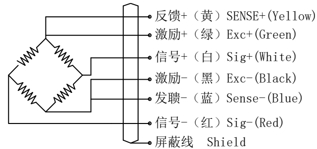
Wiring Schematic Diagram
