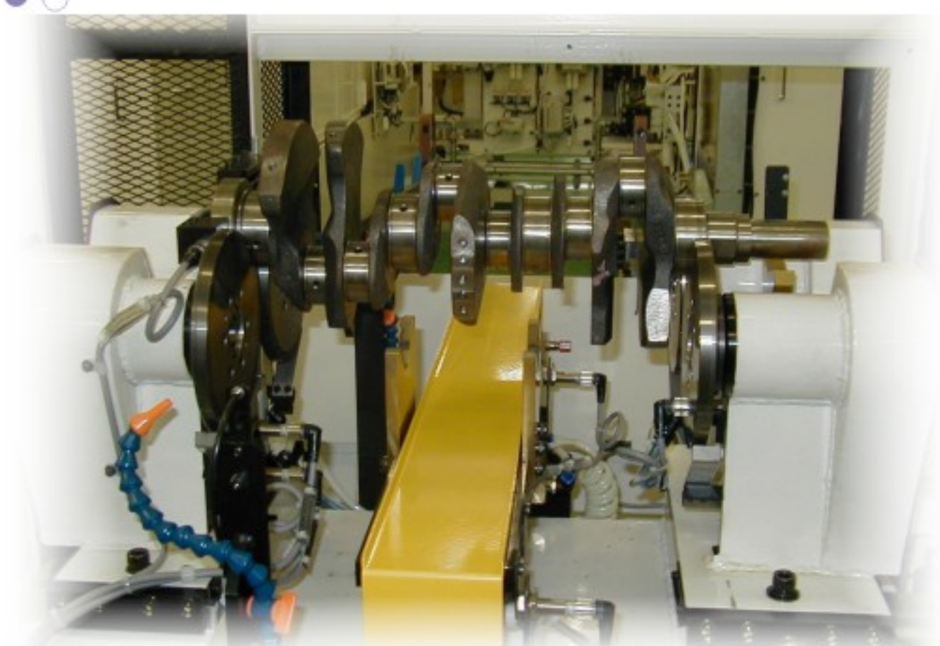
曲轴平衡机 crankshaft balancing machine
