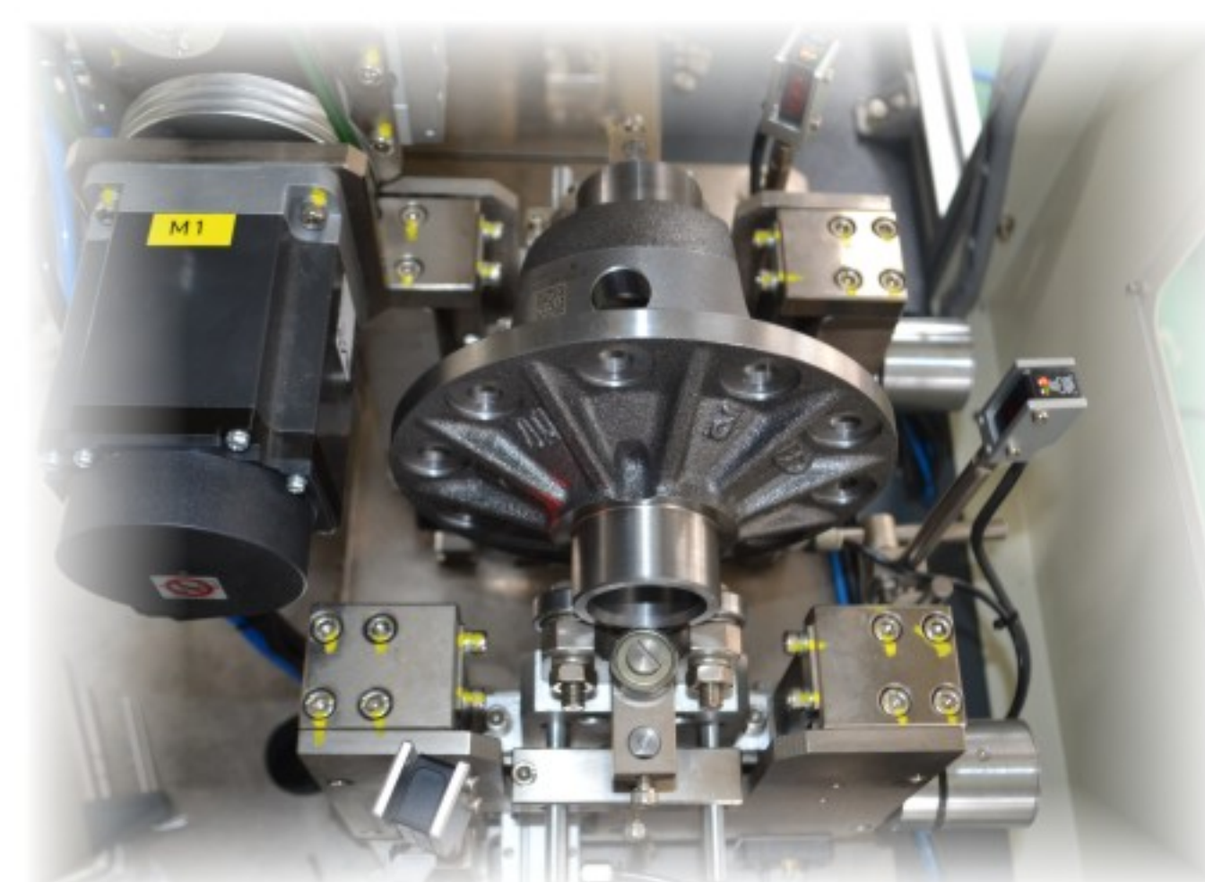
差速器平衡机 Differential balancing machine
