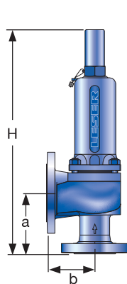
Conventional design
