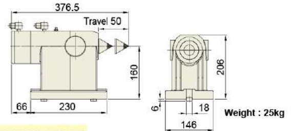
ATTJ-210/255 (With Pneumatic switching valve)
