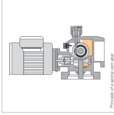
Principle of stainless steel pump head
