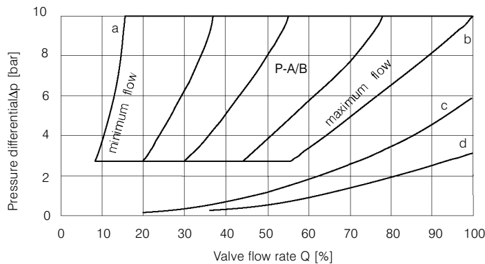
1.2.2 Figure: Pressure drop at the main spool metering edges as a function of the valve flow rate, see also table 1.2.1, p. 4
