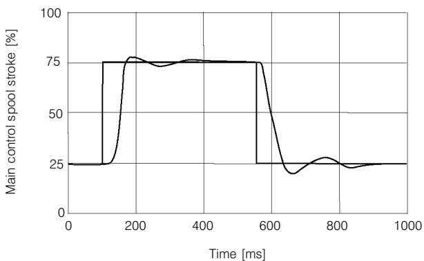
Transient function with step-shaped electrical input signal 50 % ± 25 %.
