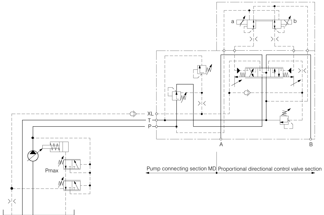
4.2.1 Figure: Example of circuit for separate actuator pressure protection in an MD valve
