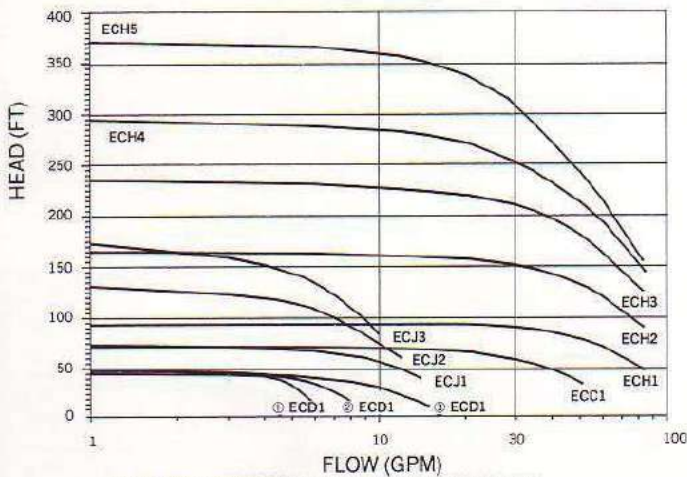
MODEL ECD1 PORT SIZES: ① (1/4" x 1/4") ② (1/2" x 1/4") ③ (1/2" x 3/8")
