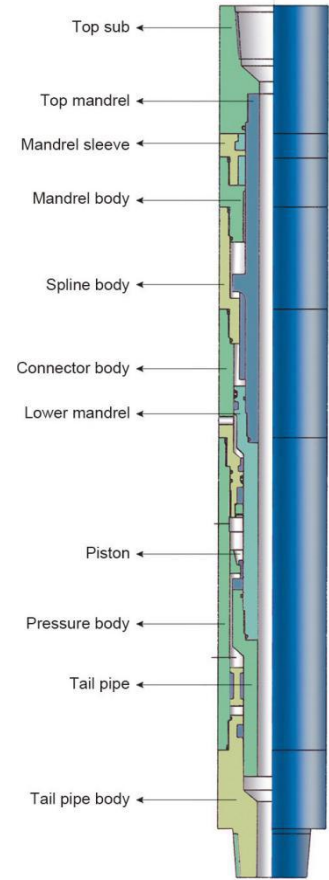
CSJ Super Fishing Jar
