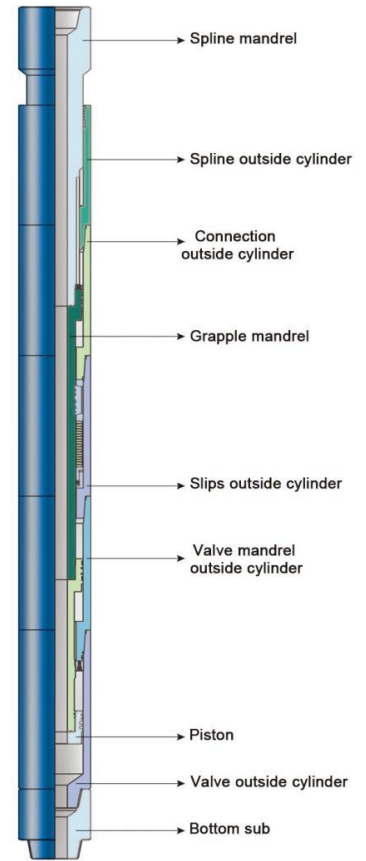
JYSZ Double Acting Hydraulic-Mechanical Drilling Jar
