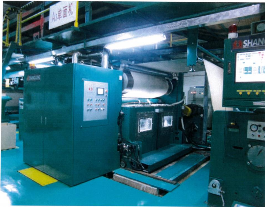
SHANG LUNG CASSETTE TYPE SINGLE FACER ( CSF-300)
