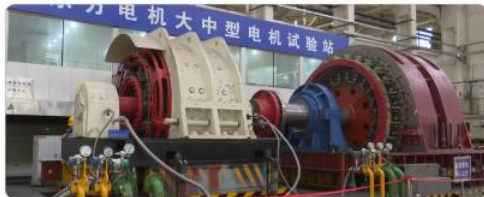
21000kW, 182r/min大低速风洞电机 2,1000kW, 182r/min large low speed wind tunnel motor
